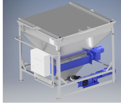
Servi Monsterkvern
