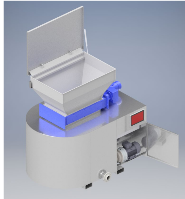
2000 liters kverntank.
